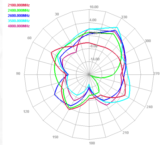
H plane
