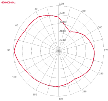
600 MHz E plane
