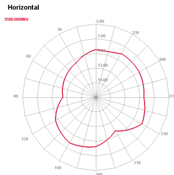
3500 MHz H plane
