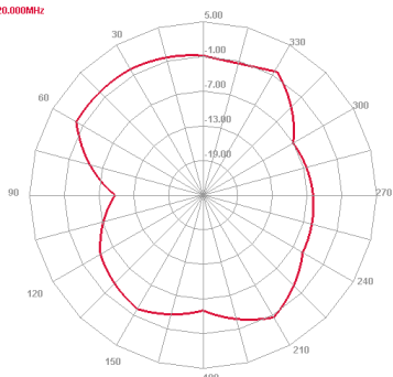
7120 MHz E plane
