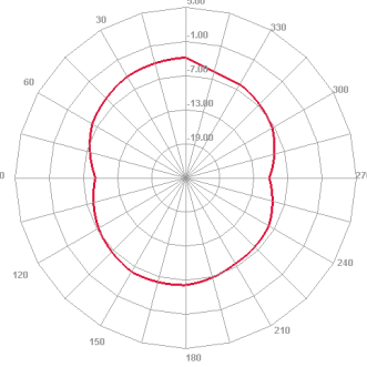
600 MHz H plane
