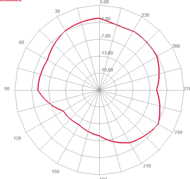
1800 MHz H plane
