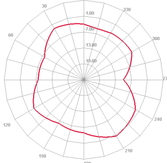
1800 MHz H plane
