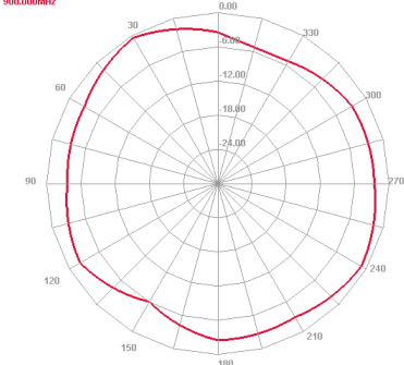
900 MHz E plane
