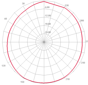
900 MHz H plane
