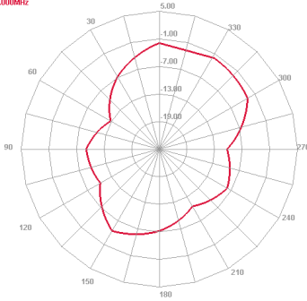
600 MHz E plane
