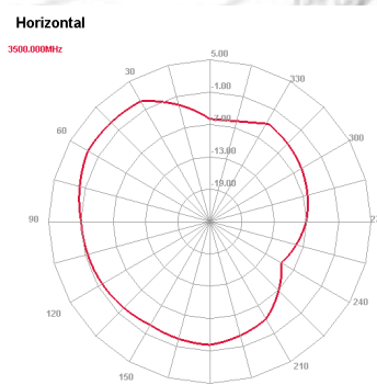
3500 MHz H plane
