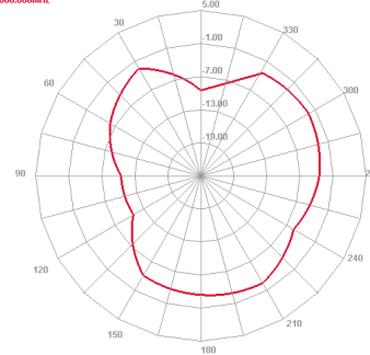
6000 MHz H plane
