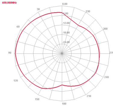
600 MHz H plane
