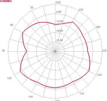
7120 MHz E plane
