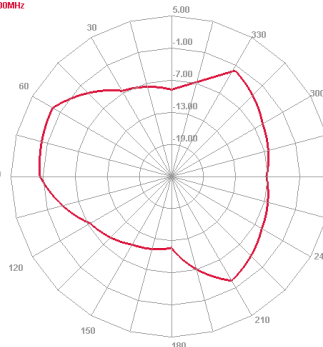
3500 MHz E plane
