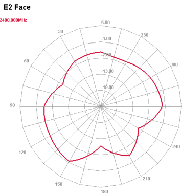
2400 MHz E plane
