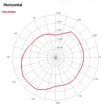
2600 MHz H plane
